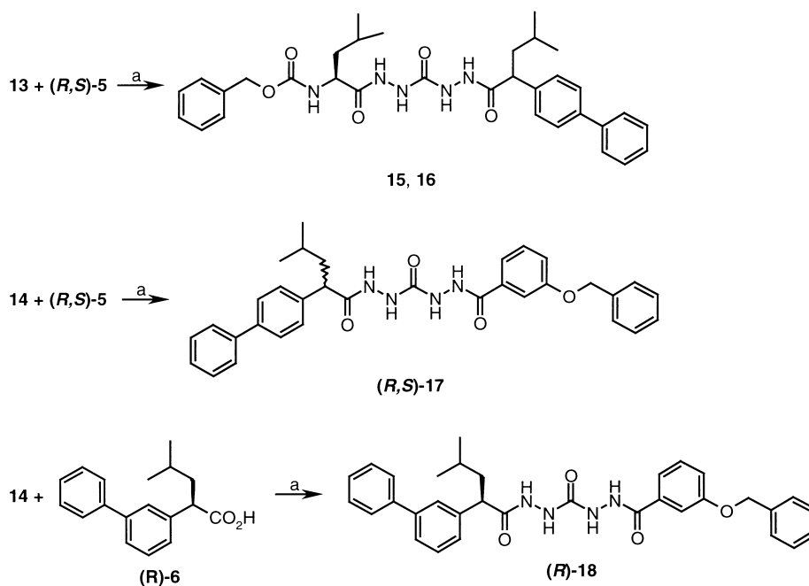
Scheme 3. (a) EDC-HCl, 1-HOBT, DMF, 15 , 16 , 42% combined; ( R,S )- 17 , 53%; ( R )- 18 , 36%.
