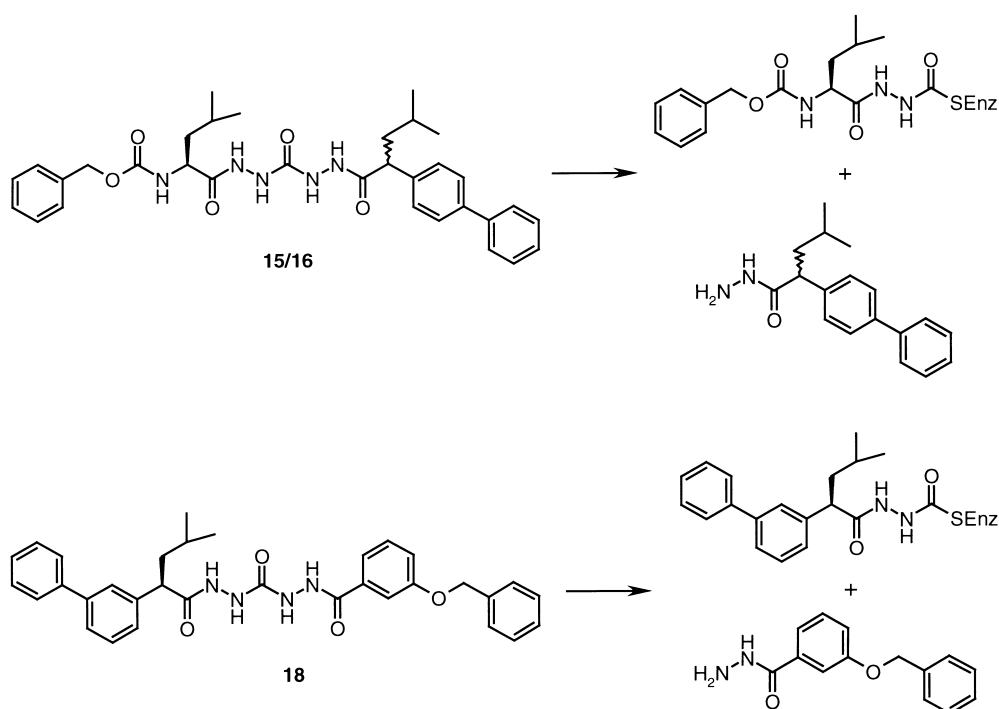
Figure 4. Products of the inhibition of cathepsin K by compounds 15/16 and compound 18 .
