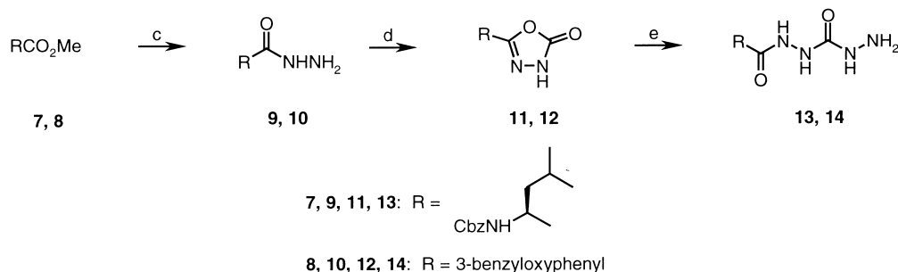
Scheme 2. (a) Benzyl chloroformate, Na 2 CO 3 , 1,4-dioxane/H 2 O, 100%; (b) benzyl bromide, K 2 CO 3 , acetone, 98%; (c) H 2 NNH 2 ·H 2 O, MeOH, 9, 100%; 10, 94%; (d) Cl 2 CO, toluene, 110 °C; 11, 96%; 12, 96%; (e) H 2 NNH 2 ·H 2 O, MeOH, 13, 60%; 14, 93%.
