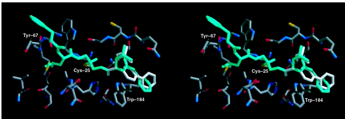
Figure 2. Stereoview of the binding model for the 2-isobutyl-4-biphenylacetyl peptidomimetic (white) superimposed with inhibitor 1 (cyan). Selected active site residues are colored by atom (C = grey, O = red, N = blue, S = yellow).
