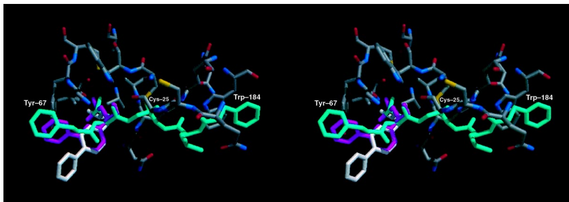
Figure 3. Stereoview of the binding models for the 2-isobutyl-4-biphenylacetyl peptidomimetic (white) and 2-isobutyl-3-biphenylacetyl peptidomimetic (magenta) superimposed with inhibitor 1 (cyan). Selected active site residues are colored by atom (C=grey, O=red, N=blue, S=yellow).
