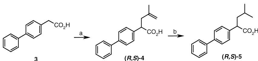
Scheme 1. (a) i. 2.2 equiv. LDA (lithium diisopropylamide), THF; ii. 3-bromo-2-methylpropene, 72%; (b) H 2 , Pd-C, EtOAc, 95%.
